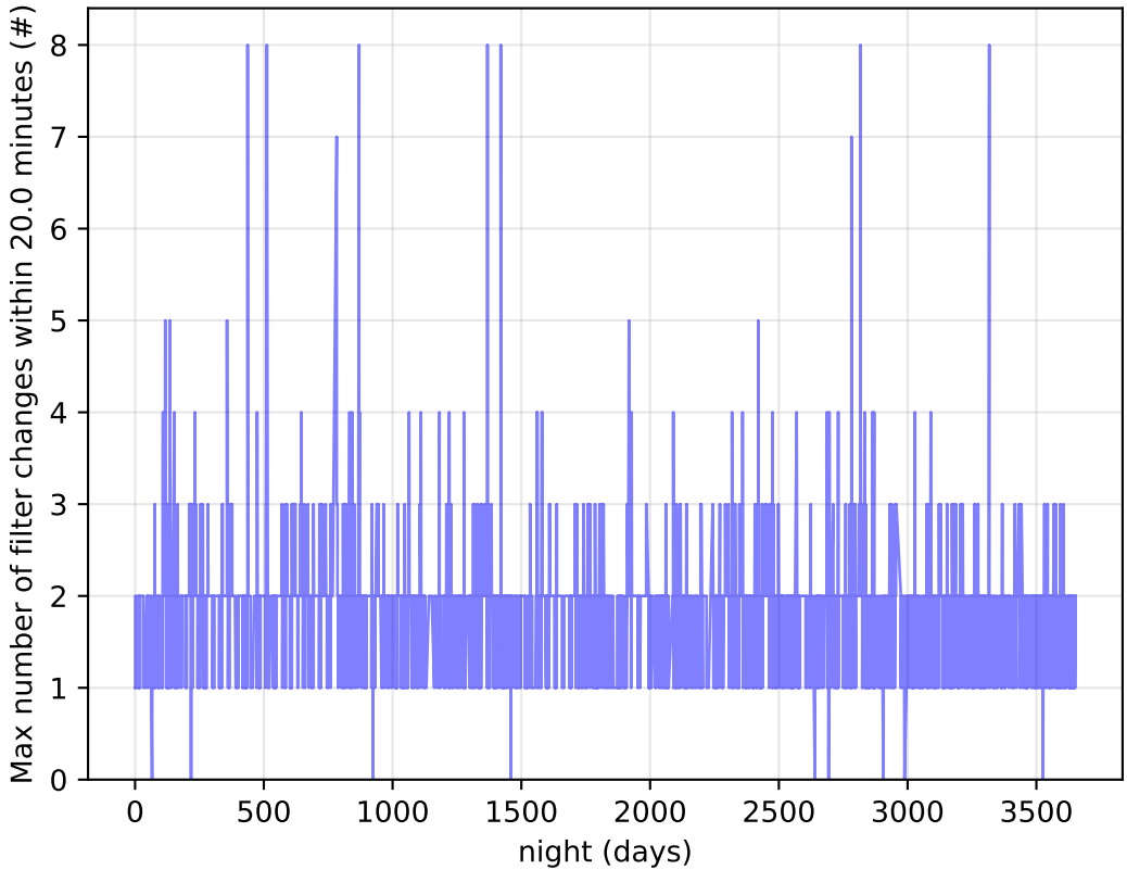
too_elab_r16_d3_gz_v3.4_10yrs Per Night: Max number of filter changes within 20.0 minutes
