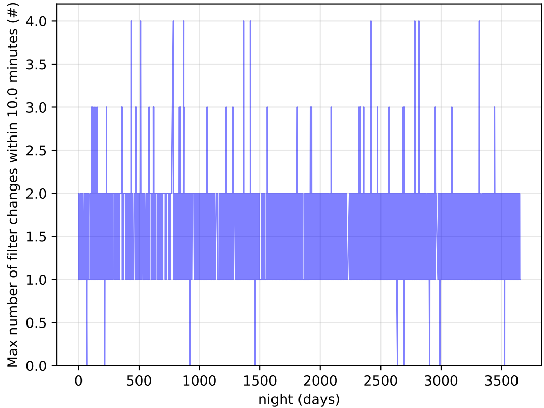
too_elab_r16_d3_gz_v3.4_10yrs Per Night: Max number of filter changes within 10.0 minutes
