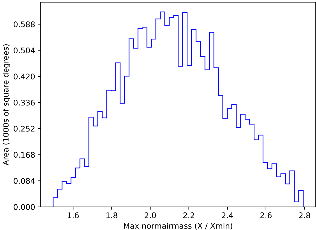
too_elab_r16_d3_gz_v3.4_10yrs WFD y band: Max normairmass
