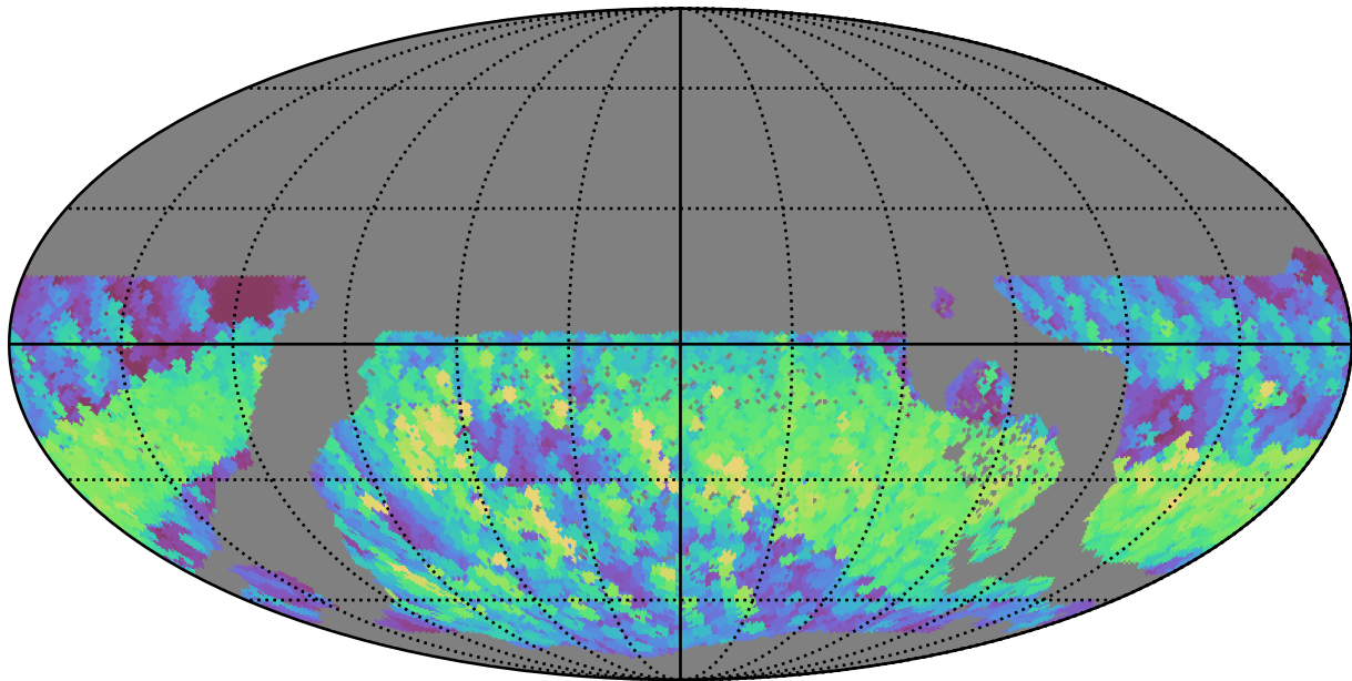
too_elab_r16_d3_gz_v3.4_10yrs WFD r band: Max normairmass
