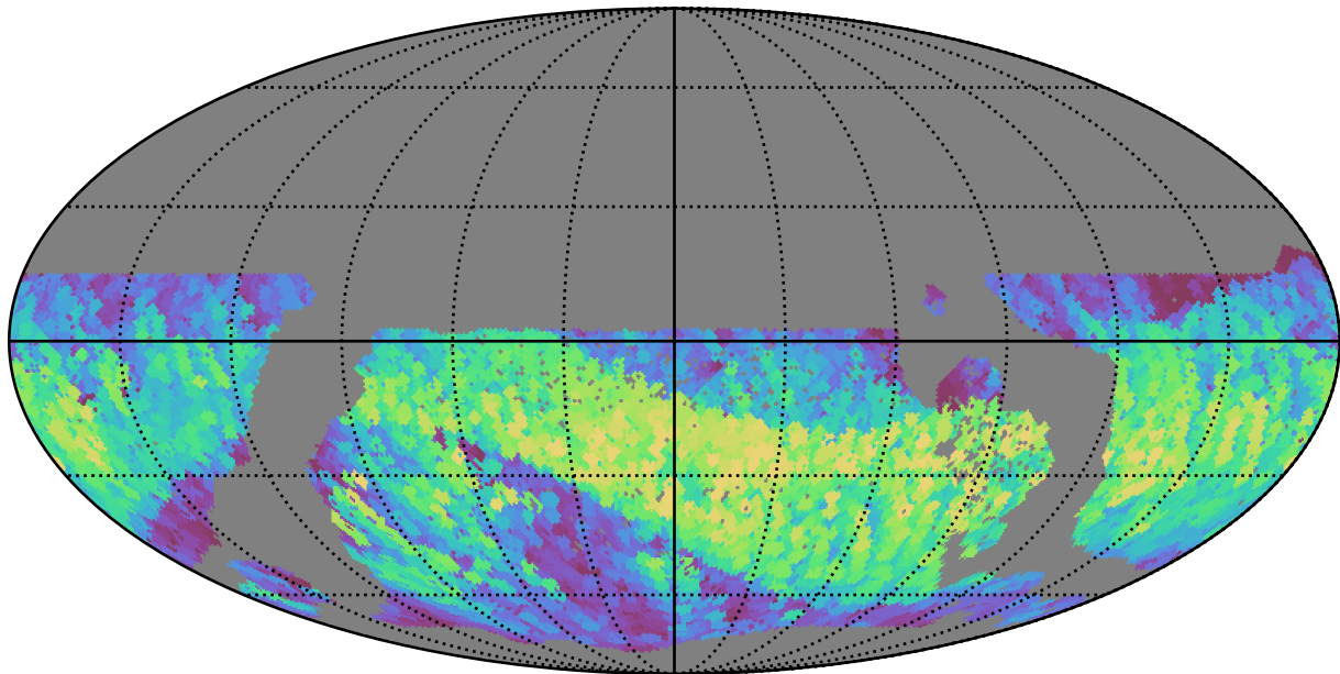
too_elab_r16_d3_gz_v3.4_10yrs WFD i band: Max normairmass
