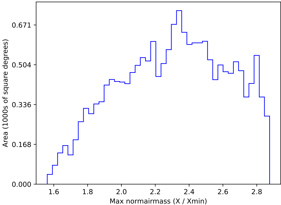
too_elab_r16_d3_gz_v3.4_10yrs WFD i band: Max normairmass
