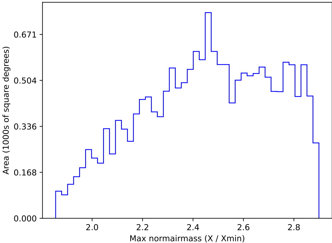
too_elab_r16_d3_gz_v3.4_10yrs WFD all bands: Max normairmass
