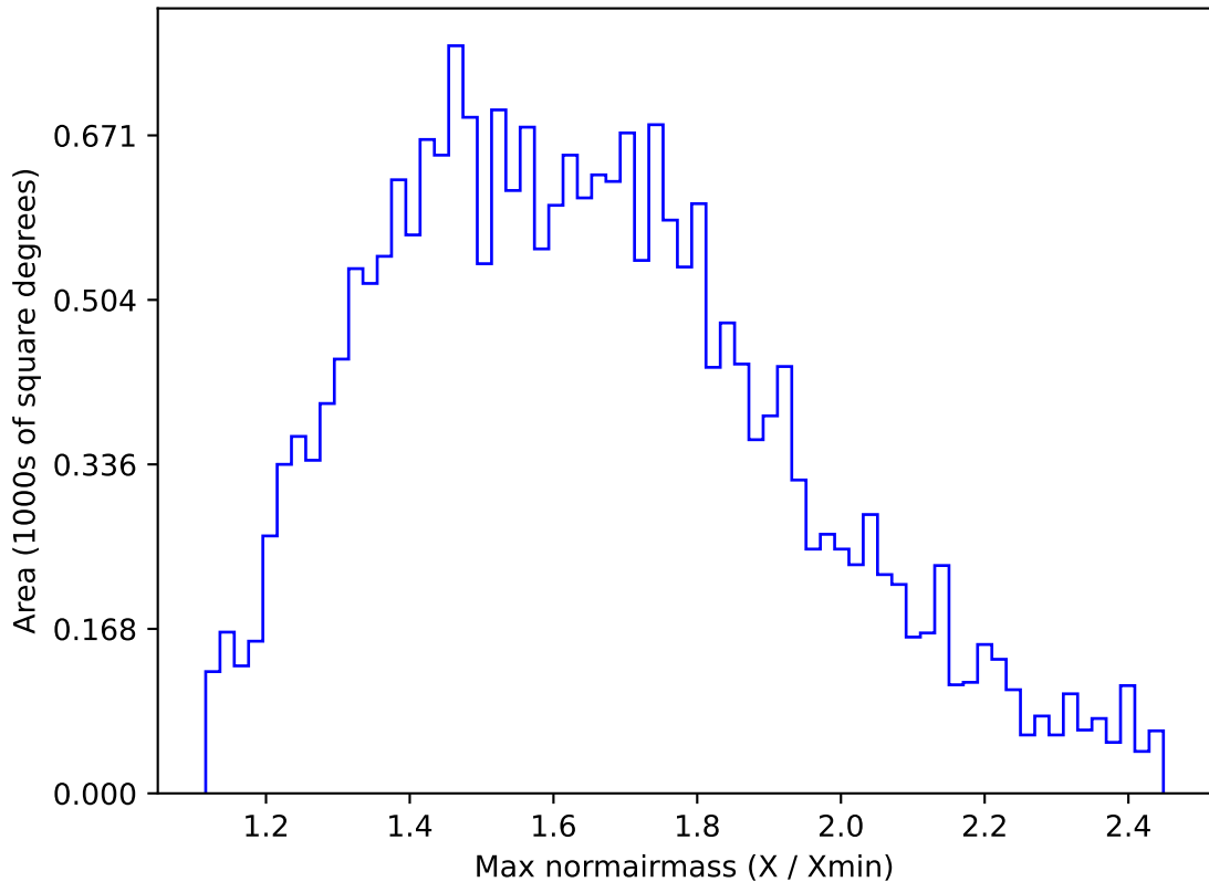
too_elab_r16_d3_gz_v3.4_10yrs All sky u band: Max normairmass
