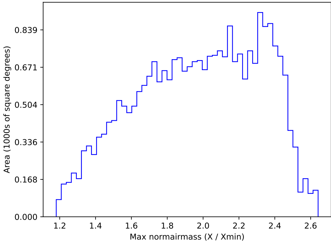
too_elab_r16_d3_gz_v3.4_10yrs All sky r band: Max normairmass
