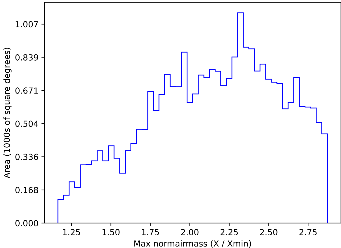
too_elab_r16_d3_gz_v3.4_10yrs All sky i band: Max normairmass
