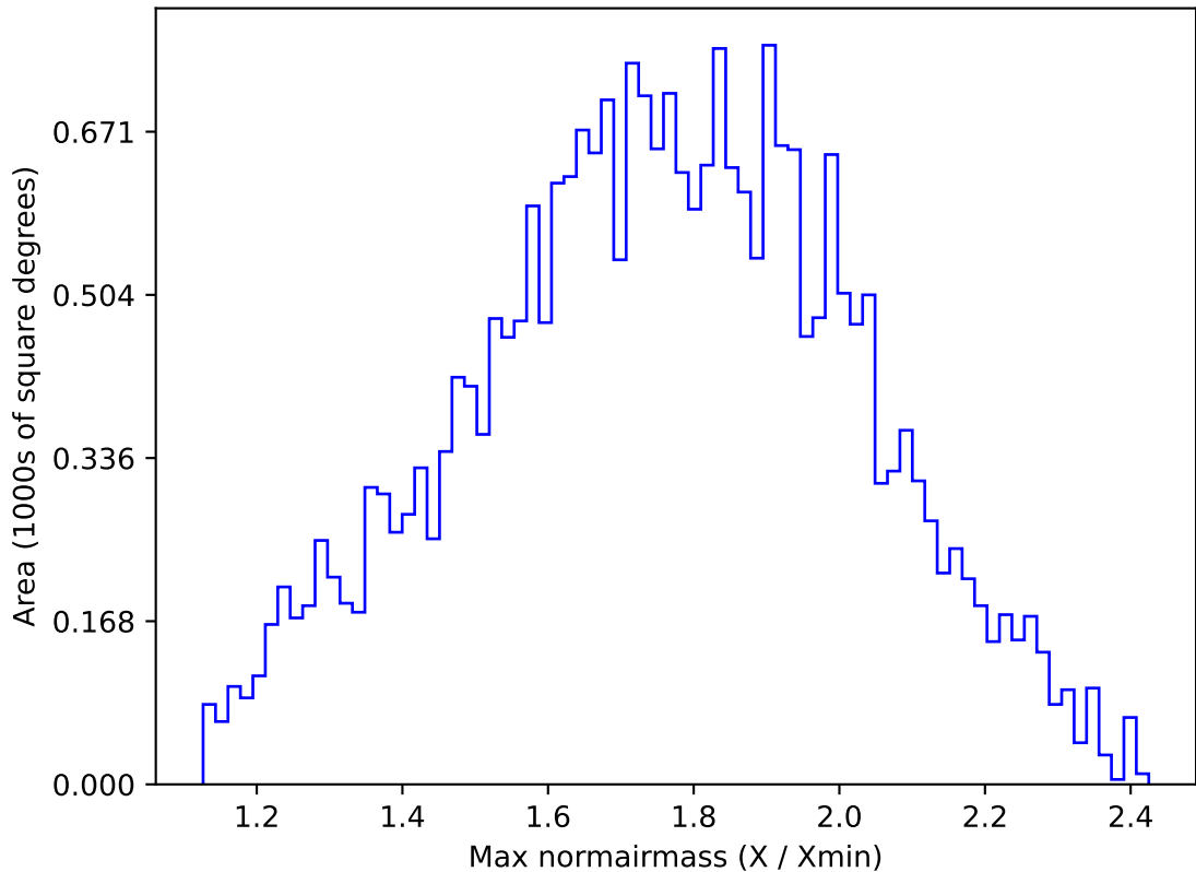
too_elab_r16_d3_gz_v3.4_10yrs All sky g band: Max normairmass
