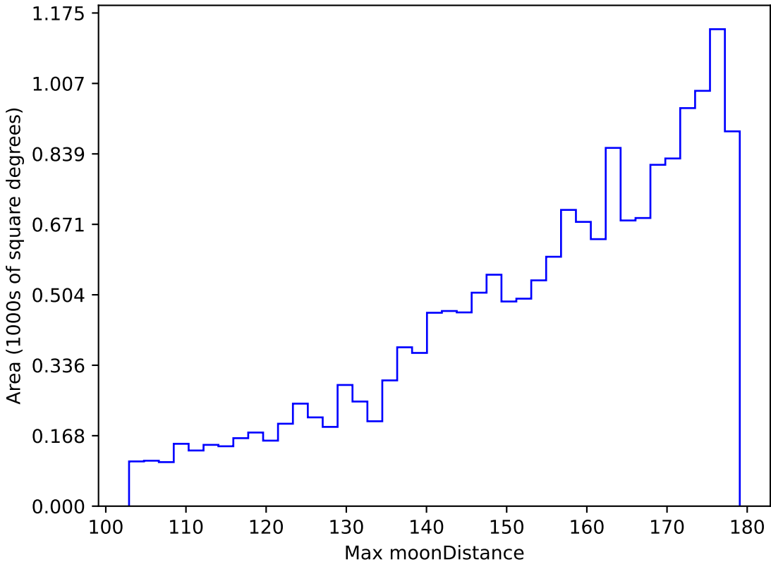
too_elab_r16_d3_gz_v3.4_10yrs WFD z band: Max moonDistance
