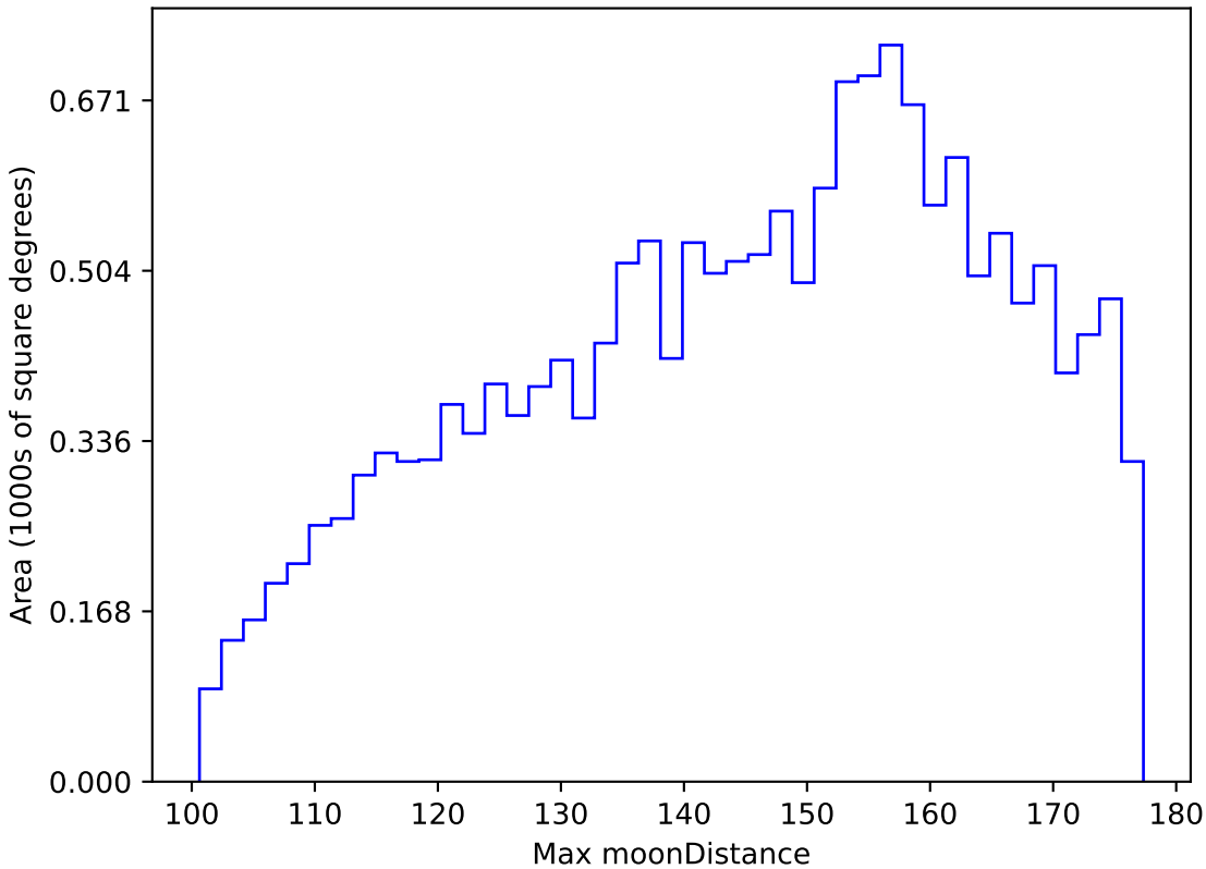
too_elab_r16_d3_gz_v3.4_10yrs WFD y band: Max moonDistance
