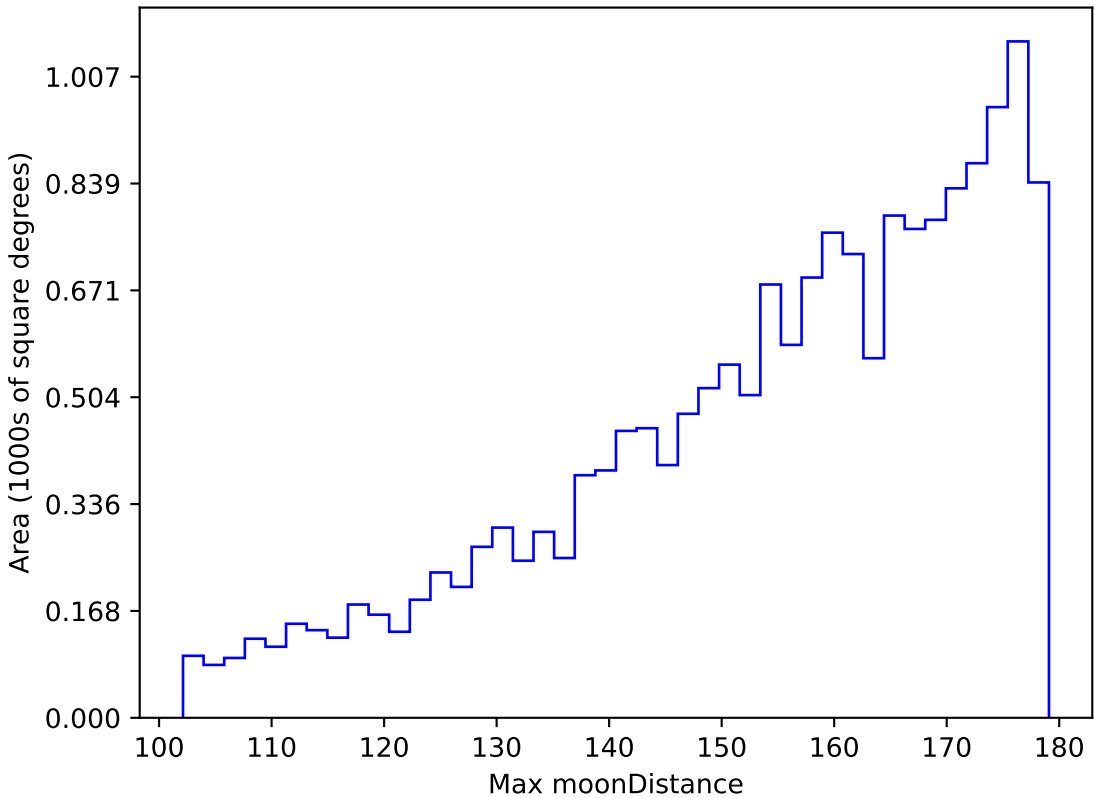
too_elab_r16_d3_gz_v3.4_10yrs WFD u band: Max moonDistance
