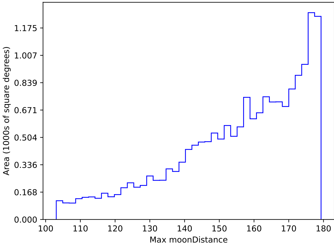
too_elab_r16_d3_gz_v3.4_10yrs WFD i band: Max moonDistance
