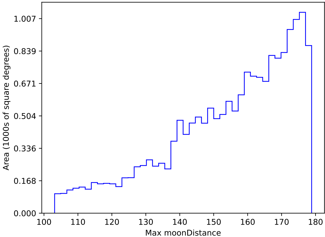
too_elab_r16_d3_gz_v3.4_10yrs WFD g band: Max moonDistance
