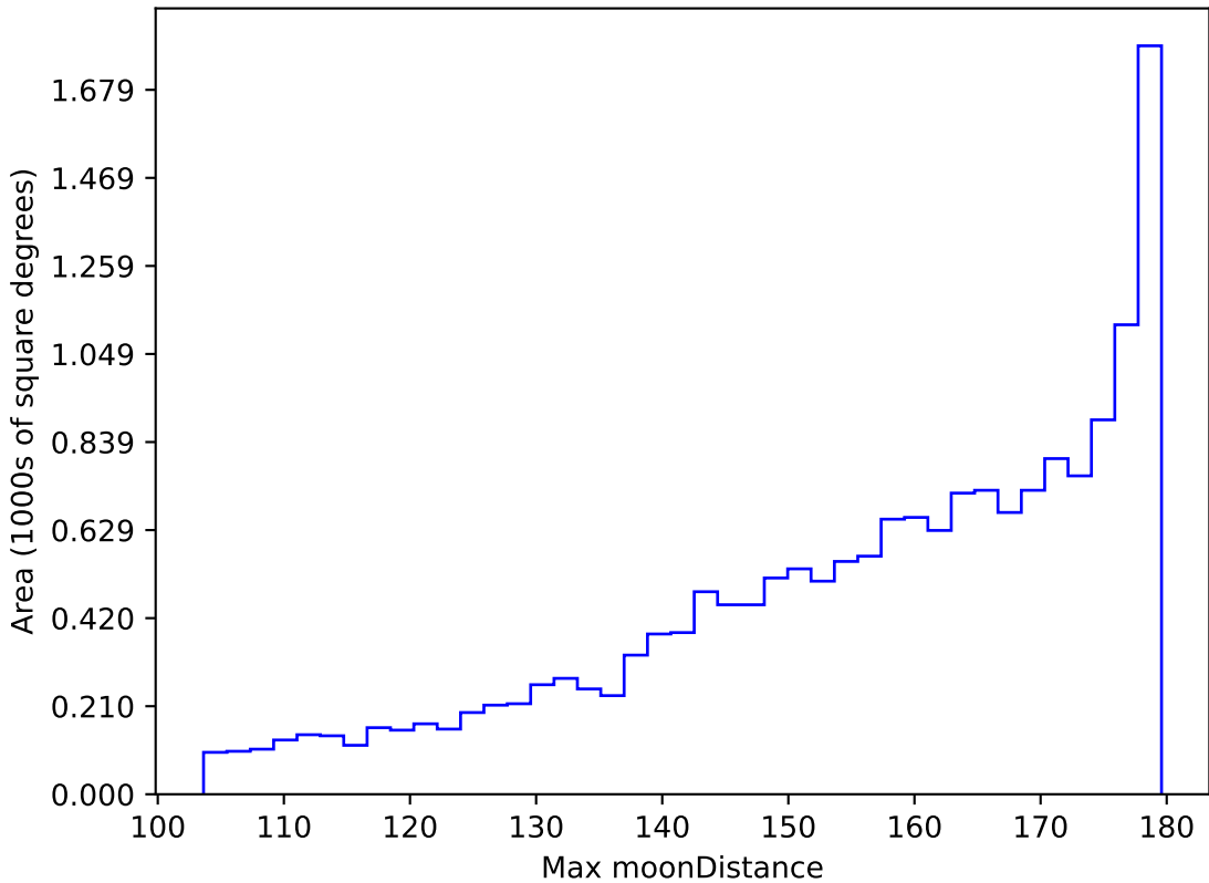
too_elab_r16_d3_gz_v3.4_10yrs WFD all bands: Max moonDistance
