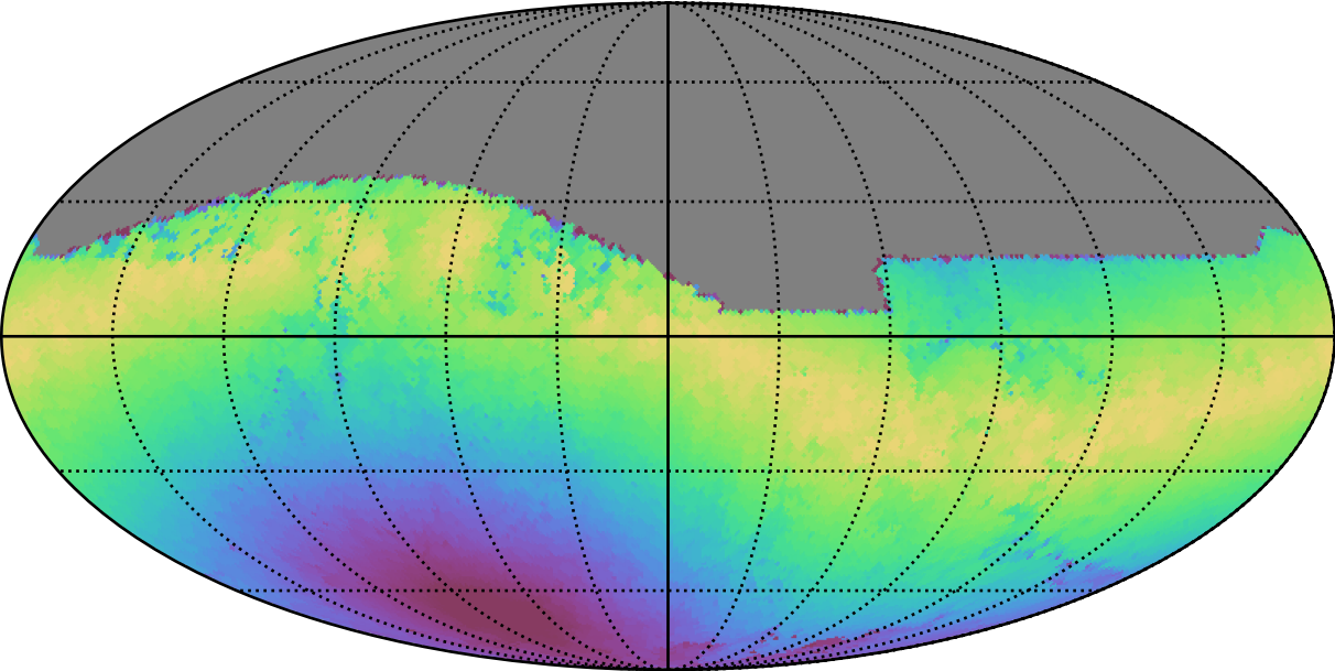
too_elab_r16_d3_gz_v3.4_10yrs All sky z band: Max moonDistance
