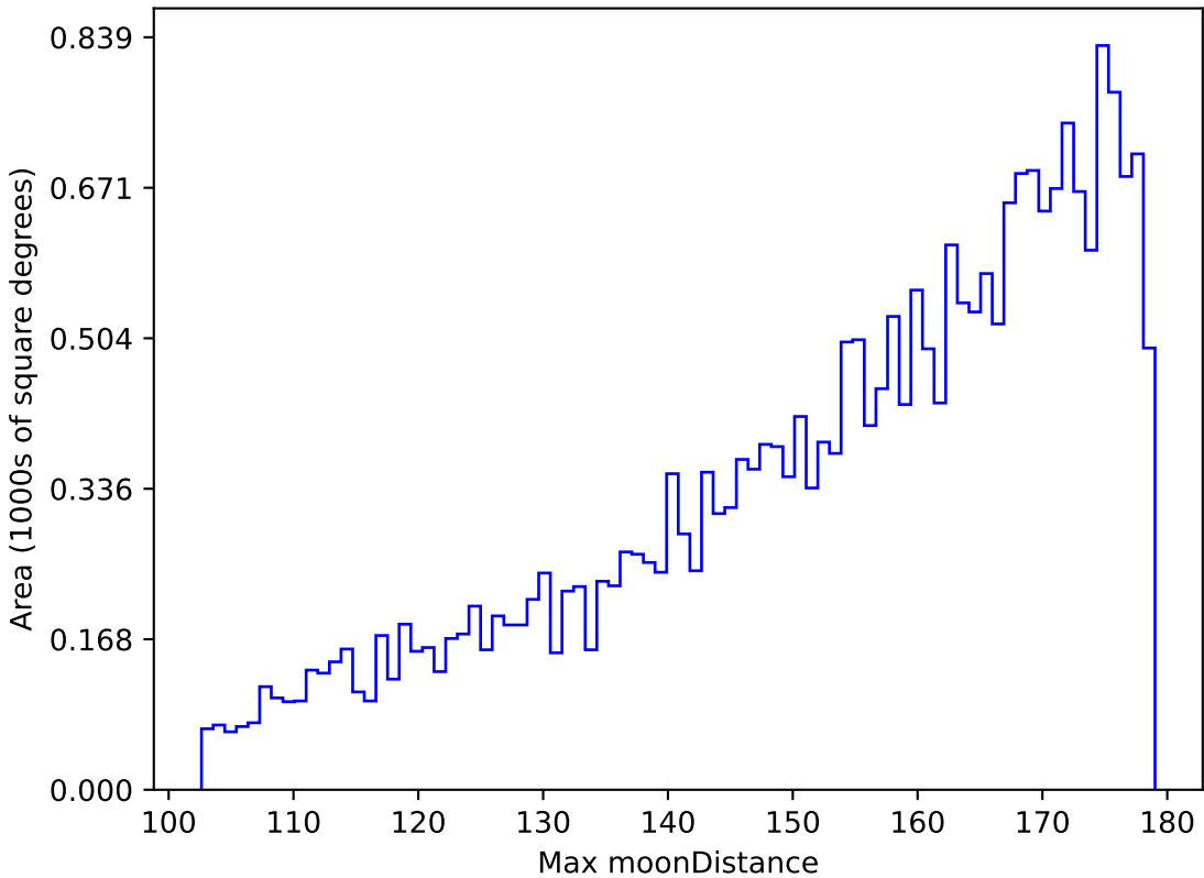
too_elab_r16_d3_gz_v3.4_10yrs All sky z band: Max moonDistance
