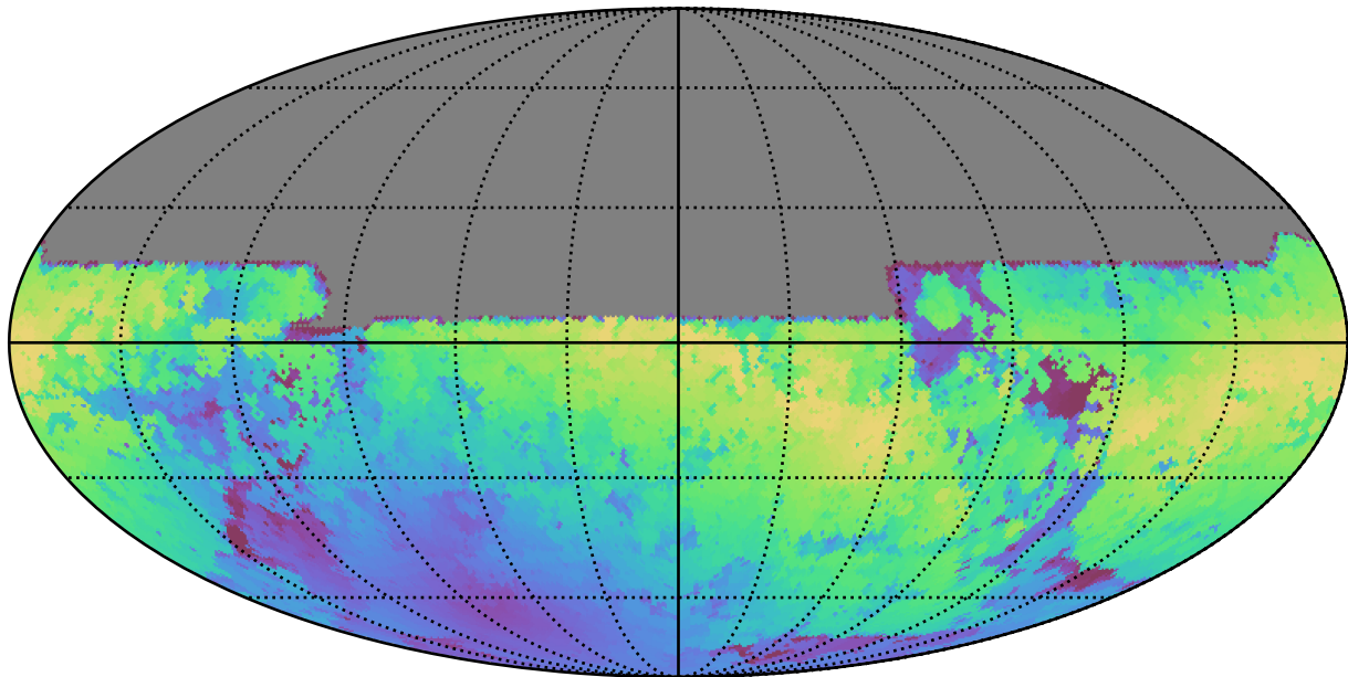
too_elab_r16_d3_gz_v3.4_10yrs All sky y band: Max moonDistance
