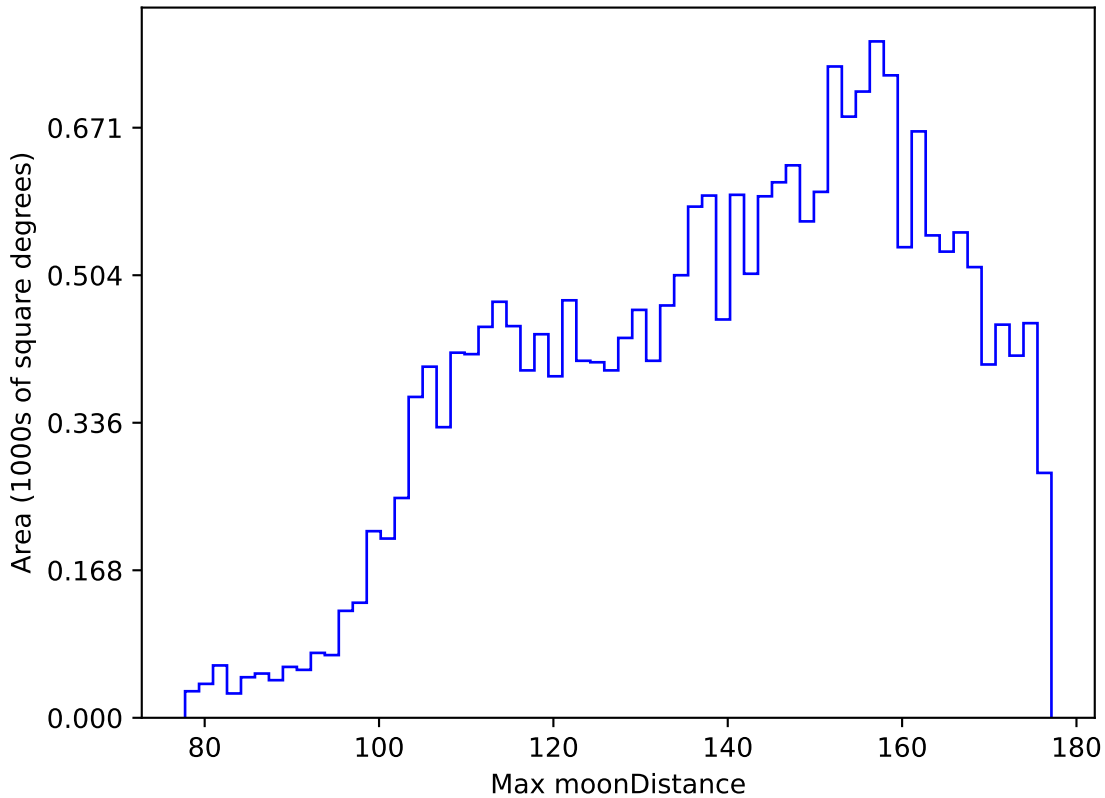
too_elab_r16_d3_gz_v3.4_10yrs All sky y band: Max moonDistance
