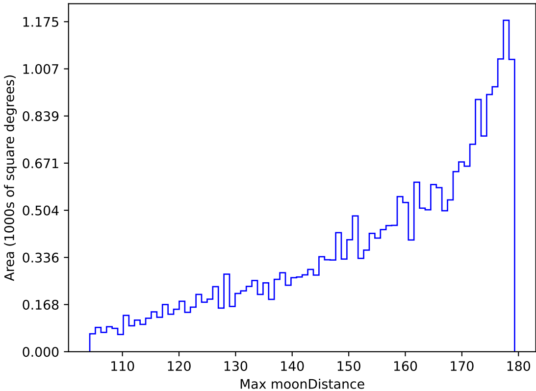
too_elab_r16_d3_gz_v3.4_10yrs All sky r band: Max moonDistance
