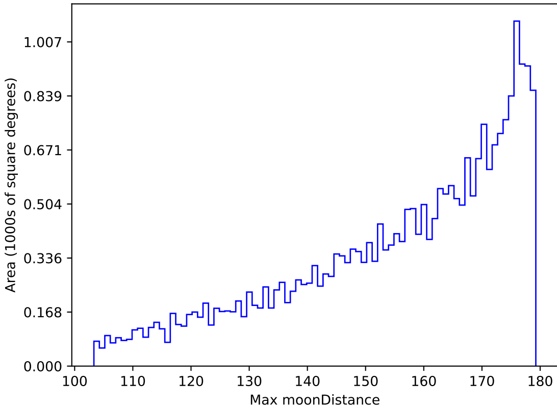
too_elab_r16_d3_gz_v3.4_10yrs All sky i band: Max moonDistance
