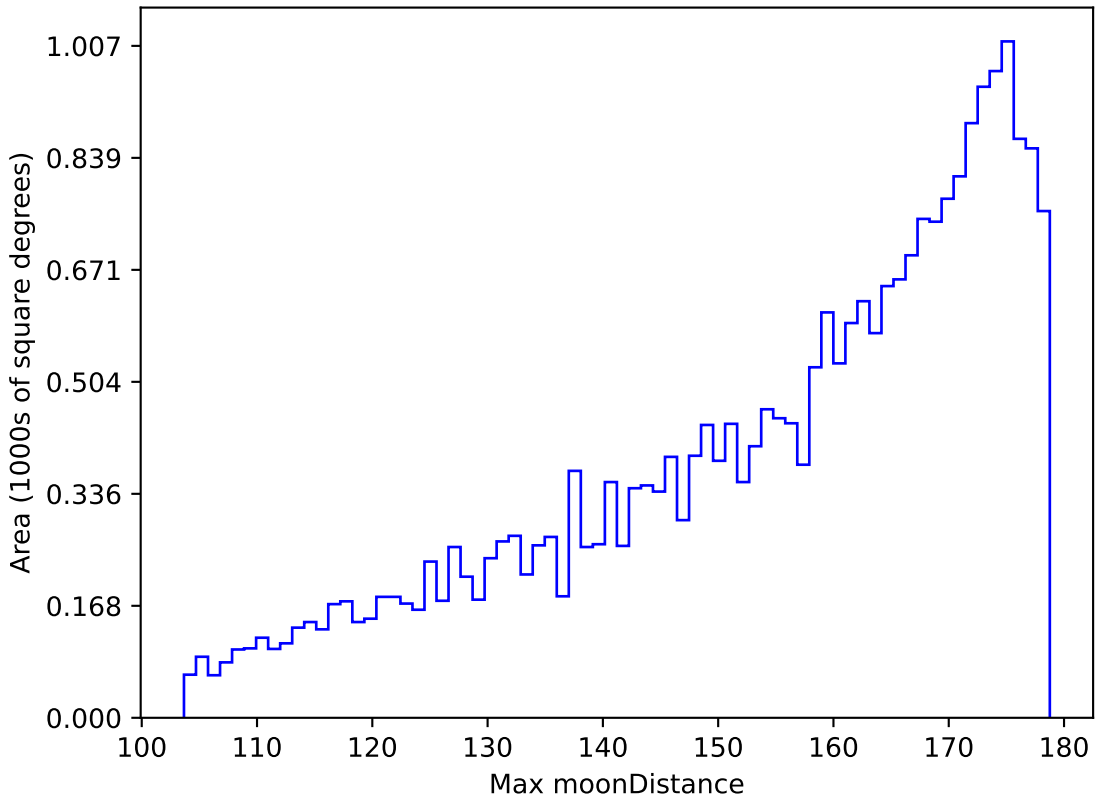
too_elab_r16_d3_gz_v3.4_10yrs All sky g band: Max moonDistance
