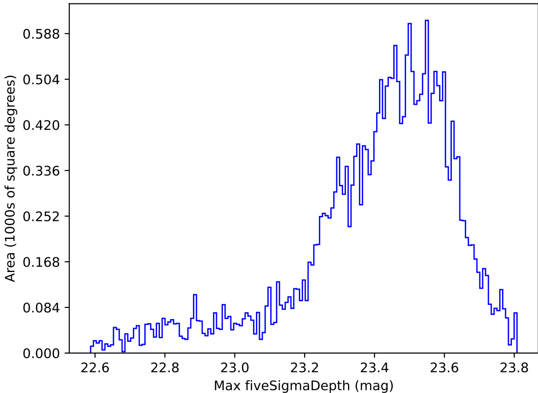
too_elab_r16_d3_gz_v3.4_10yrs Yr 1 z band: Max fiveSigmaDepth
