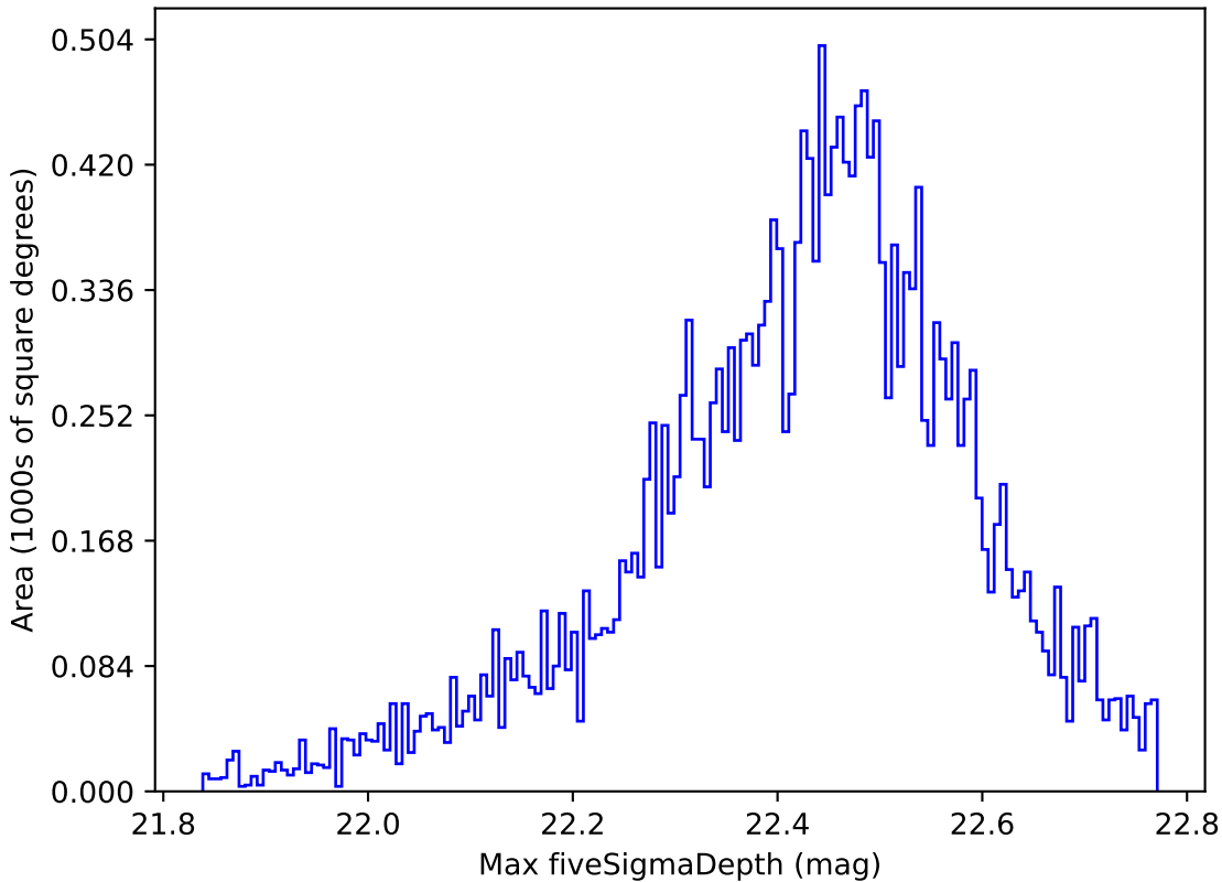
too_elab_r16_d3_gz_v3.4_10yrs Yr 1 y band: Max fiveSigmaDepth
