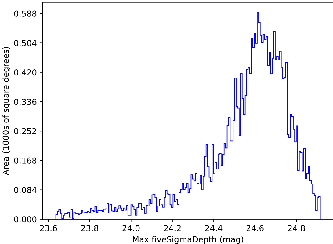
too_elab_r16_d3_gz_v3.4_10yrs Yr 1 r band: Max fiveSigmaDepth
