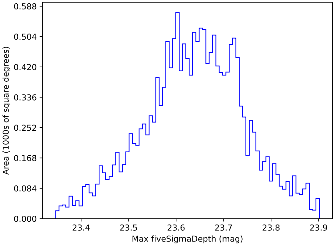
too_elab_r16_d3_gz_v3.4_10yrs WFD z band: Max fiveSigmaDepth
