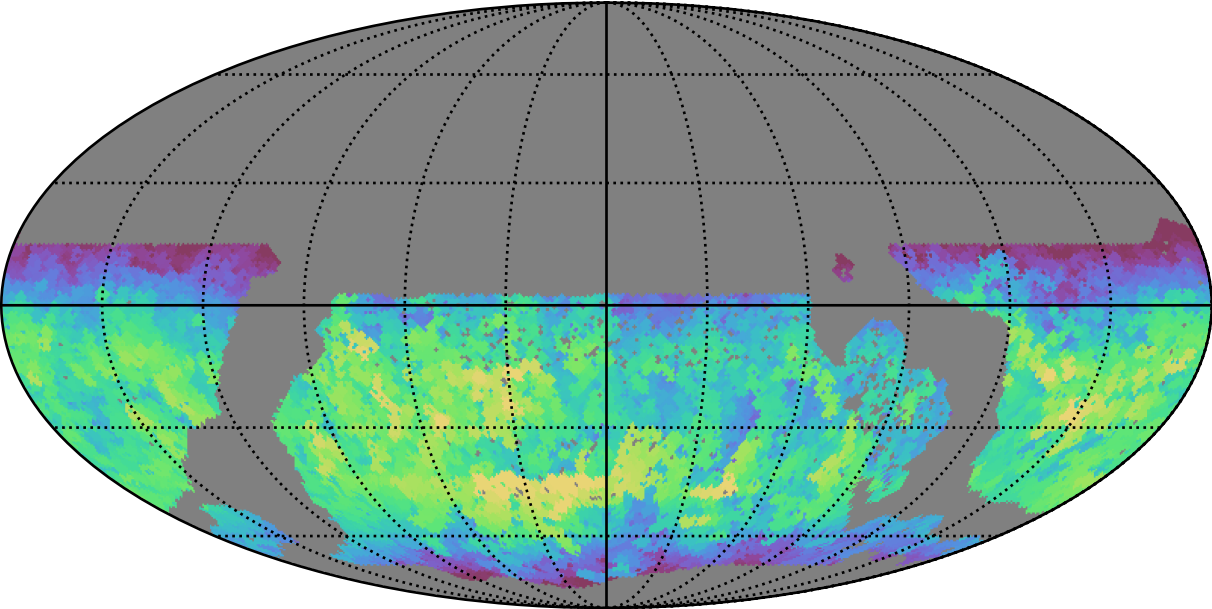
too_elab_r16_d3_gz_v3.4_10yrs WFD y band: Max fiveSigmaDepth
