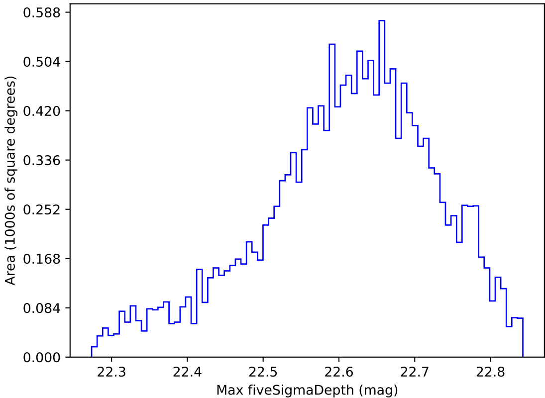
too_elab_r16_d3_gz_v3.4_10yrs WFD y band: Max fiveSigmaDepth
