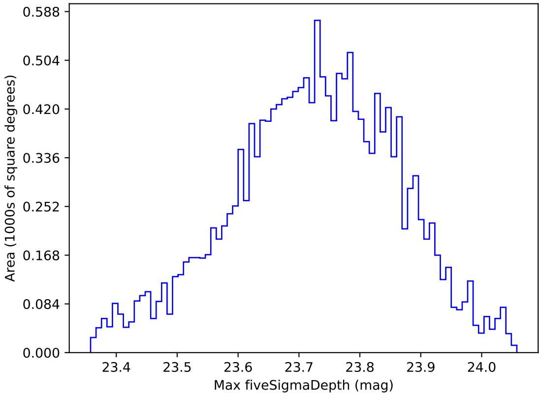
too_elab_r16_d3_gz_v3.4_10yrs WFD u band: Max fiveSigmaDepth
