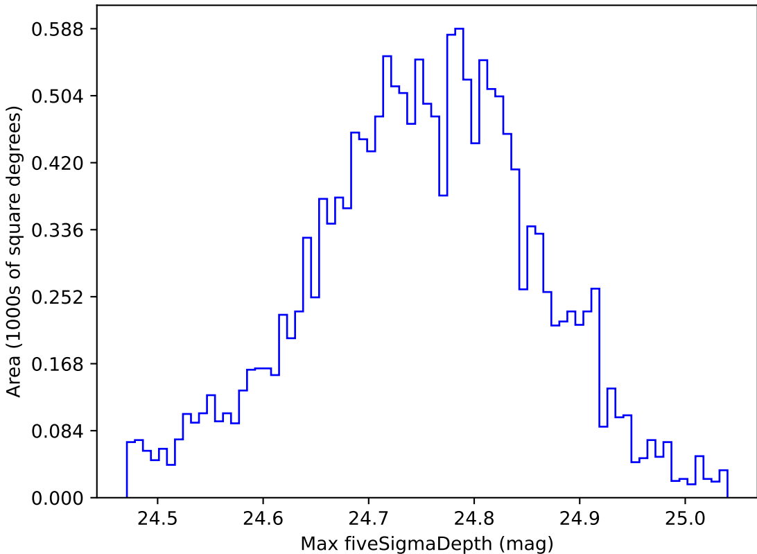
too_elab_r16_d3_gz_v3.4_10yrs WFD r band: Max fiveSigmaDepth
