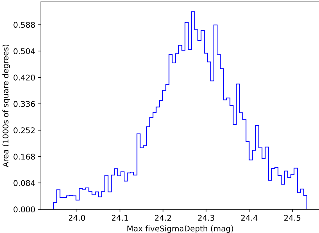
too_elab_r16_d3_gz_v3.4_10yrs WFD i band: Max fiveSigmaDepth
