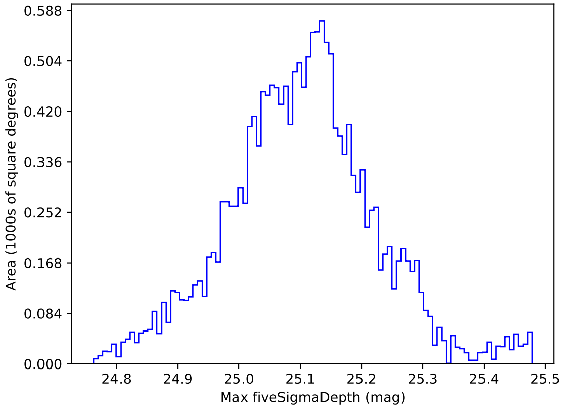
too_elab_r16_d3_gz_v3.4_10yrs WFD g band: Max fiveSigmaDepth
