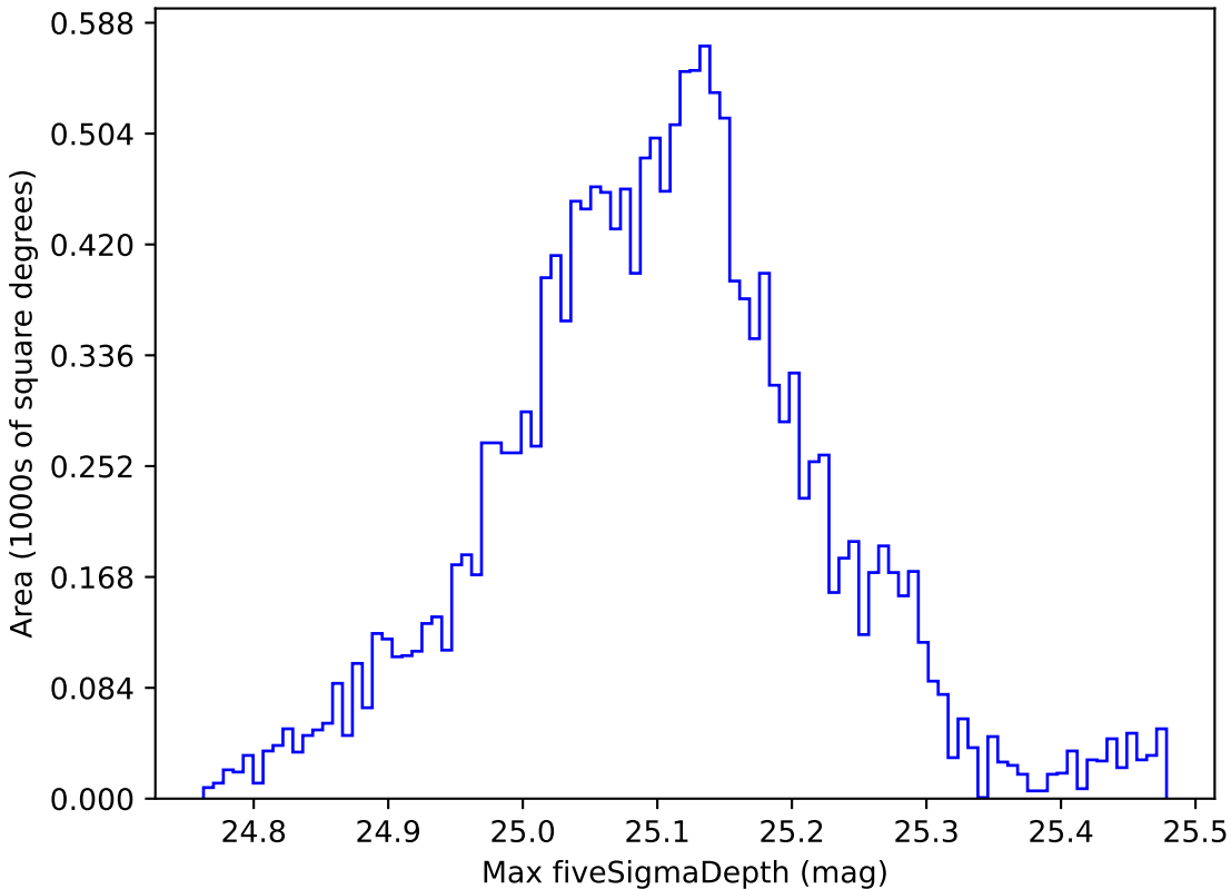
too_elab_r16_d3_gz_v3.4_10yrs WFD all bands: Max fiveSigmaDepth
