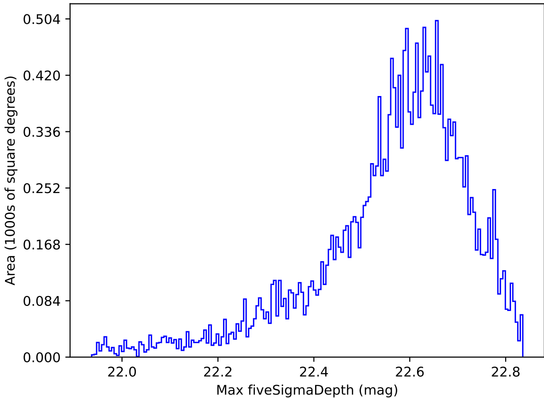
too_elab_r16_d3_gz_v3.4_10yrs All sky y band: Max fiveSigmaDepth
