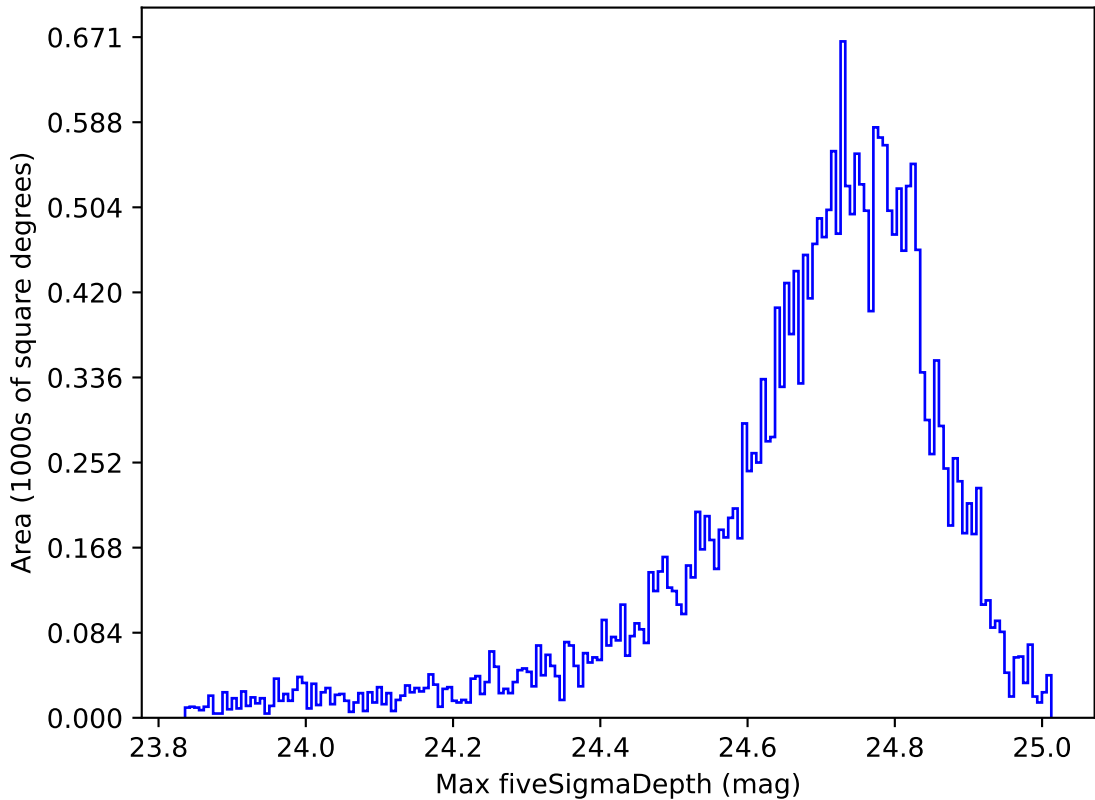
too_elab_r16_d3_gz_v3.4_10yrs All sky r band: Max fiveSigmaDepth
