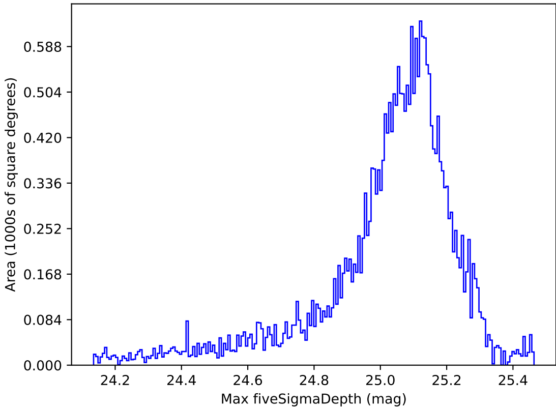
too_elab_r16_d3_gz_v3.4_10yrs All sky g band: Max fiveSigmaDepth
