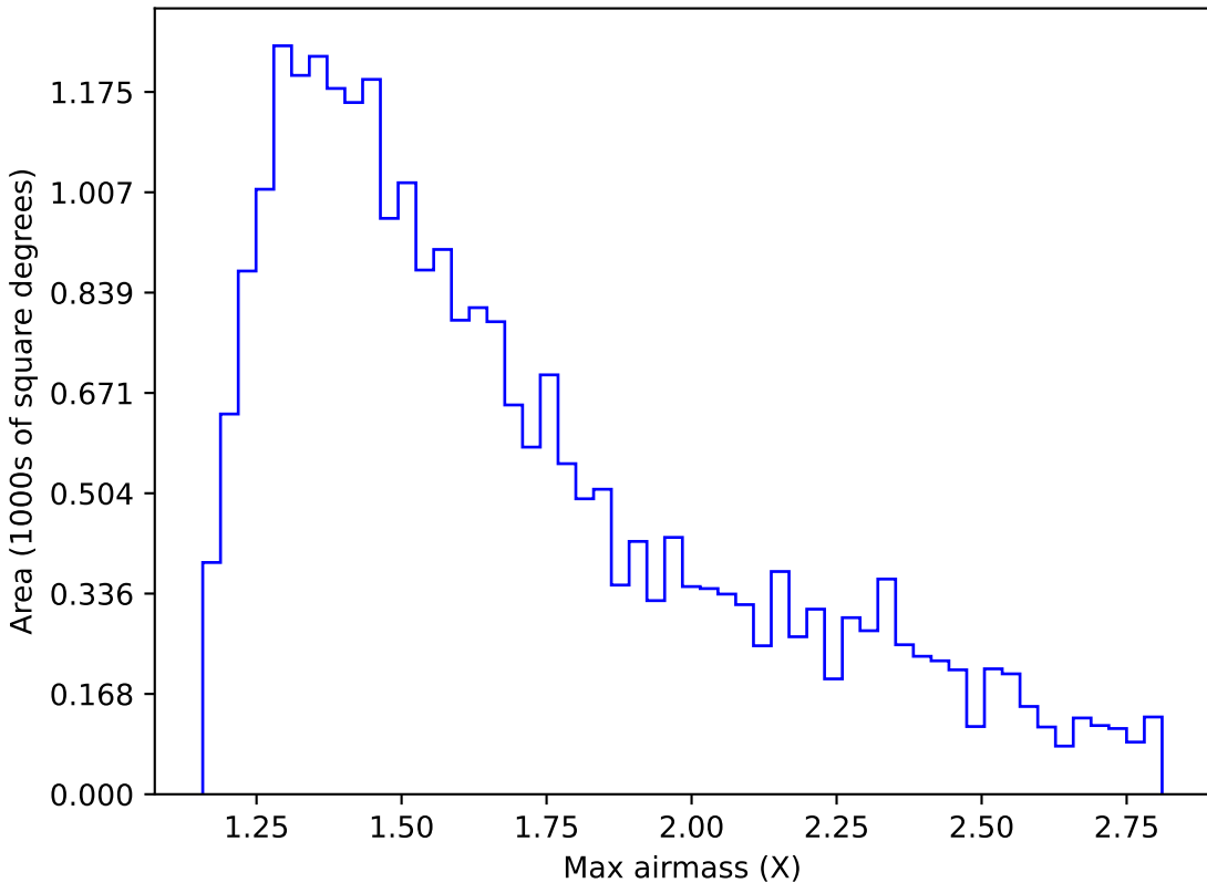
too_elab_r16_d3_gz_v3.4_10yrs Yr 1 z band: Max airmass
