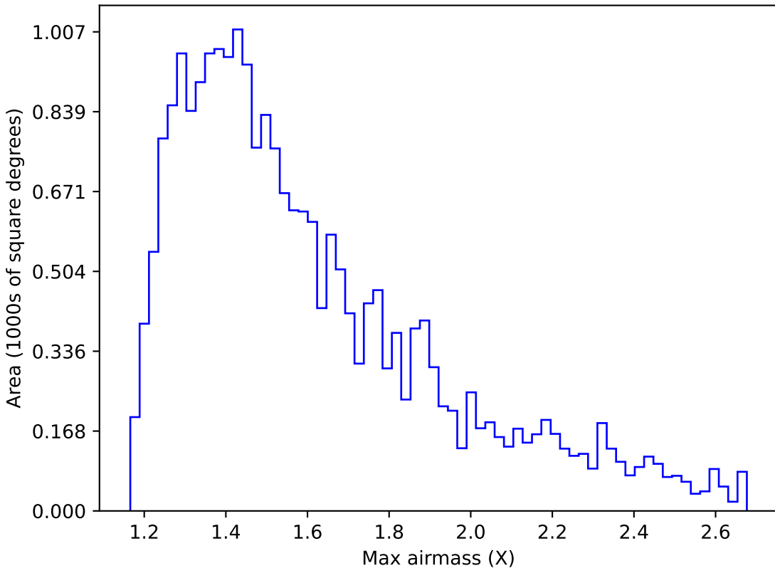
too_elab_r16_d3_gz_v3.4_10yrs Yr 1 y band: Max airmass
