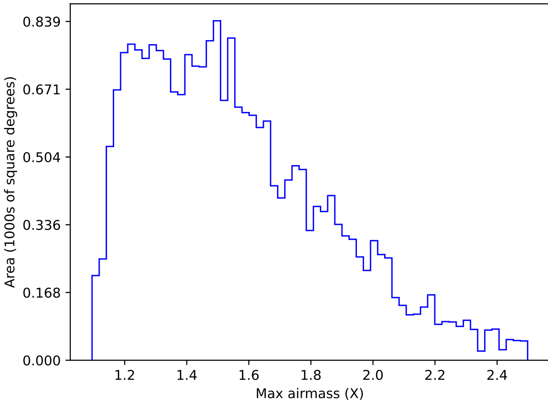
too_elab_r16_d3_gz_v3.4_10yrs Yr 1 u band: Max airmass
