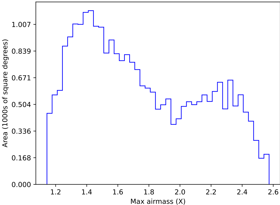
too_elab_r16_d3_gz_v3.4_10yrs Yr 1 r band: Max airmass
