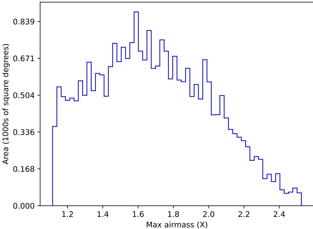
too_elab_r16_d3_gz_v3.4_10yrs Yr 1 g band: Max airmass
