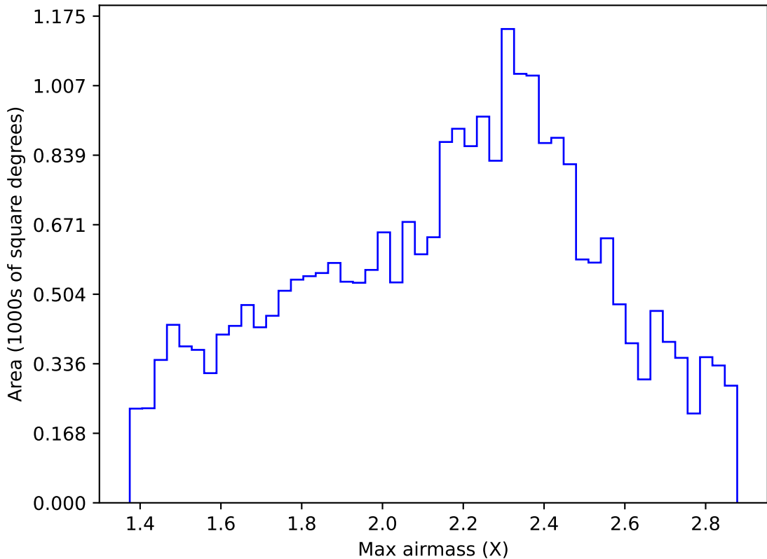
too_elab_r16_d3_gz_v3.4_10yrs Yr 1 all bands: Max airmass
