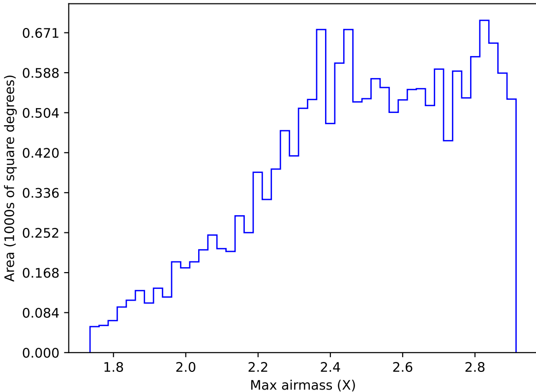
too_elab_r16_d3_gz_v3.4_10yrs WFD z band: Max airmass
