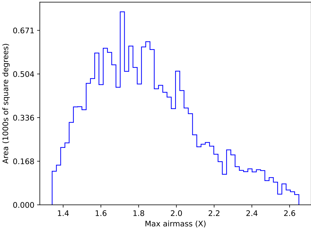
too_elab_r16_d3_gz_v3.4_10yrs WFD u band: Max airmass
