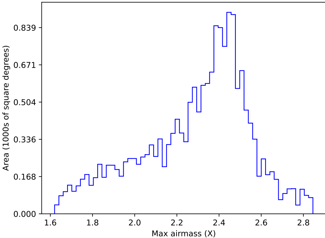
too_elab_r16_d3_gz_v3.4_10yrs WFD r band: Max airmass
