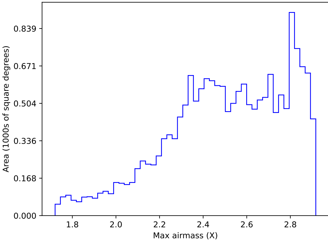
too_elab_r16_d3_gz_v3.4_10yrs WFD i band: Max airmass
