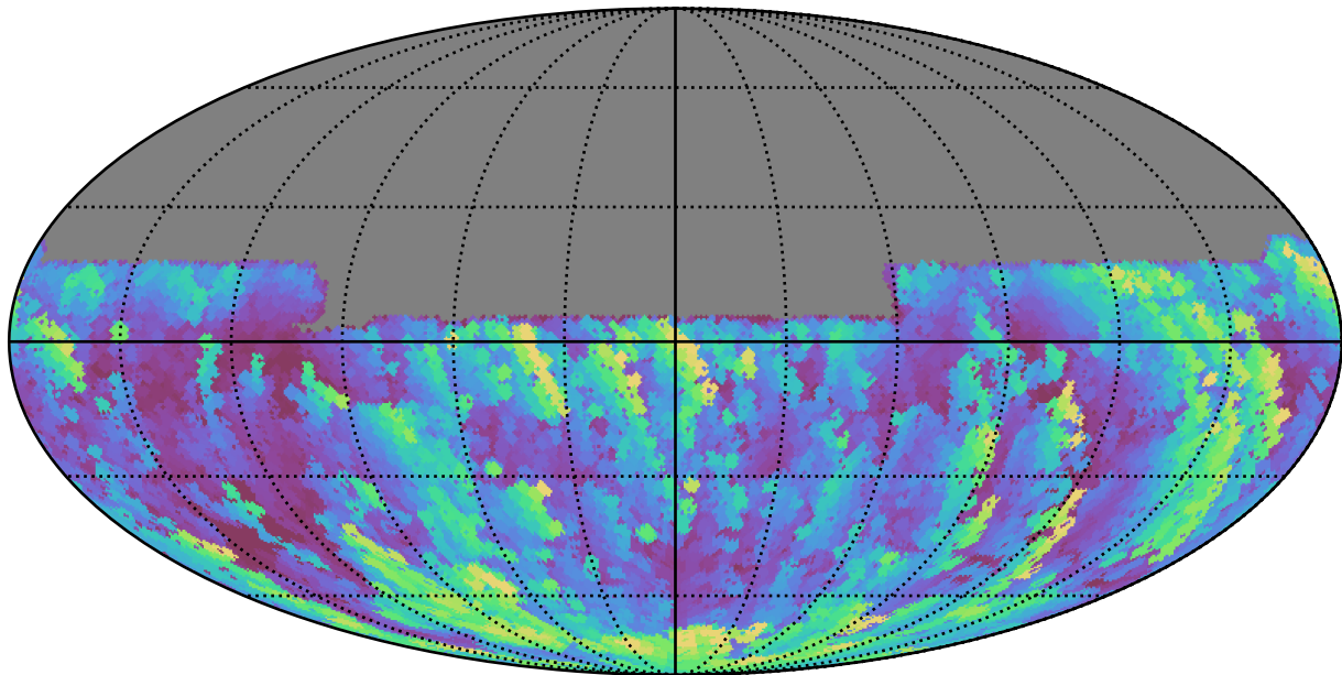
too_elab_r16_d3_gz_v3.4_10yrs All sky u band: Max airmass
