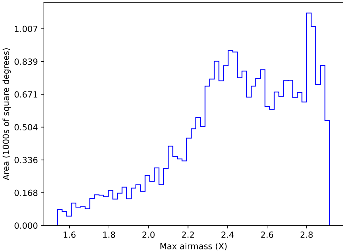
too_elab_r16_d3_gz_v3.4_10yrs All sky i band: Max airmass
